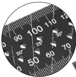
Diamond Marking Holes Ensures marking tool remains centred.
